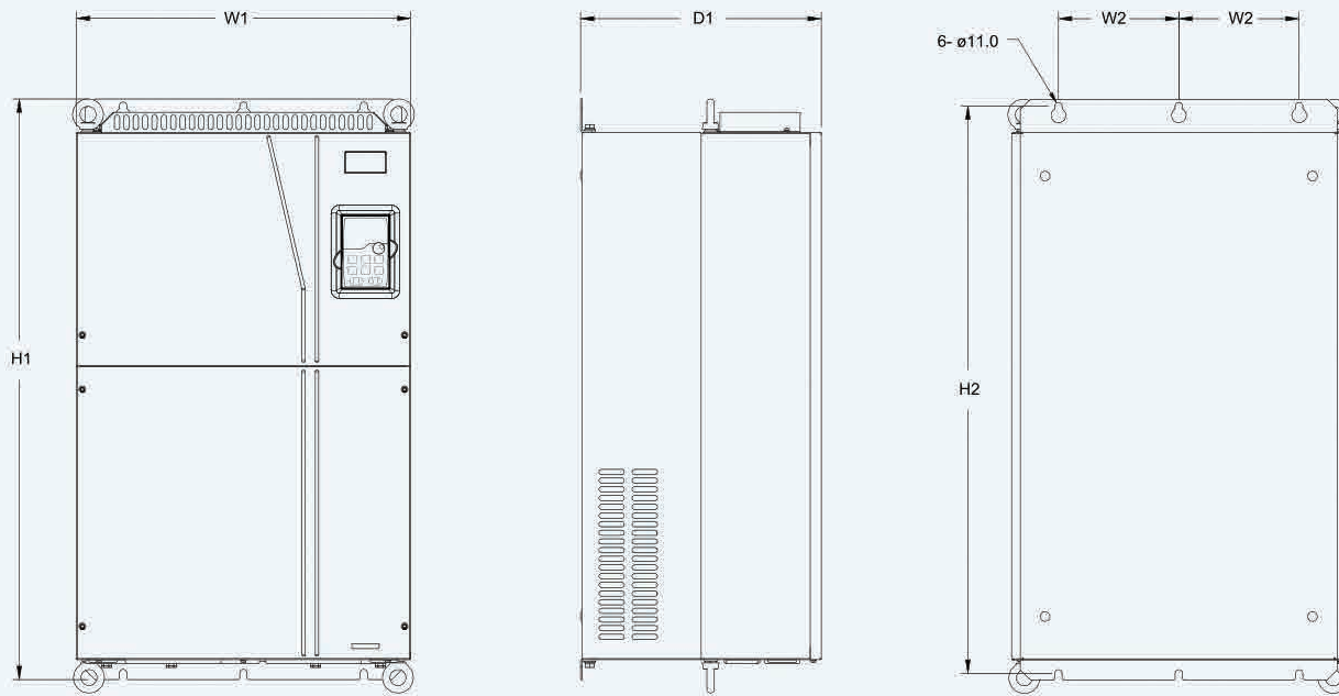
660V 160-220kW VFD wall-mounting diagram
