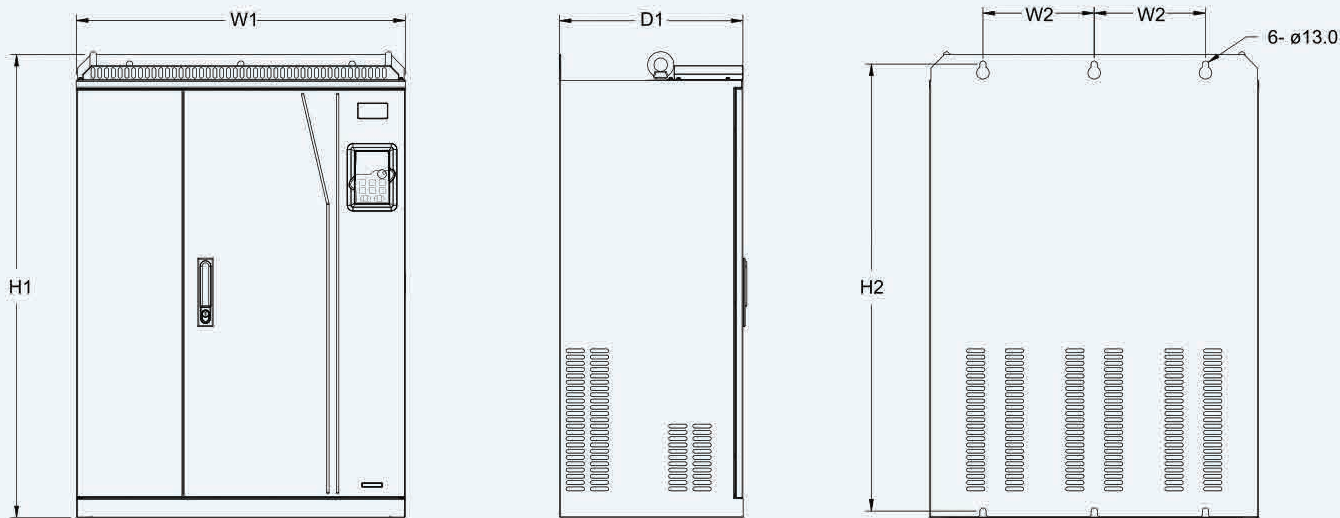
660V 250-355kW VFD wall-mounting diagram
