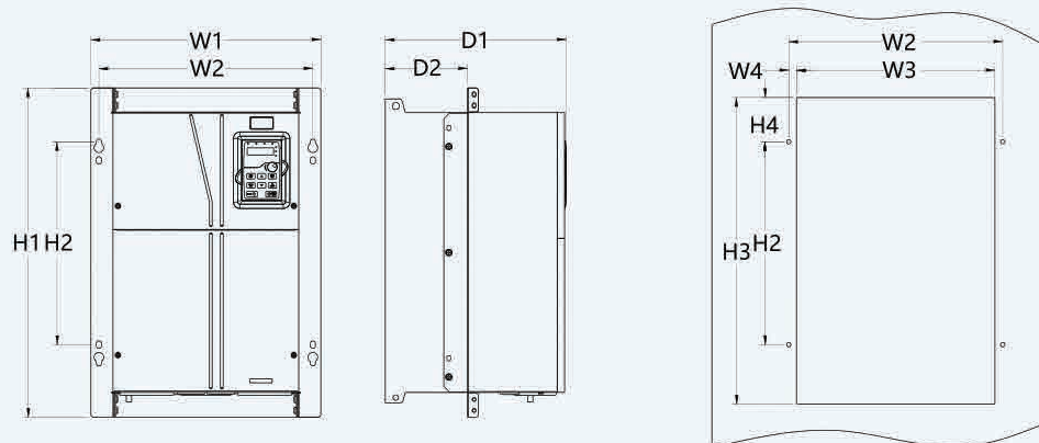
380V 90-110kW VFD flange installation diagram
