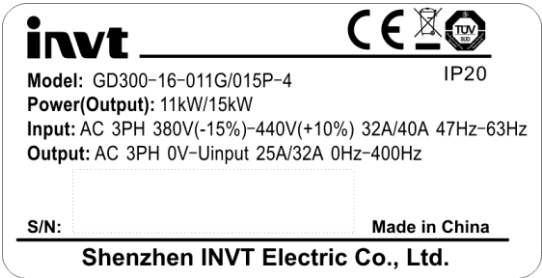
Fig 2-1 Name plate
