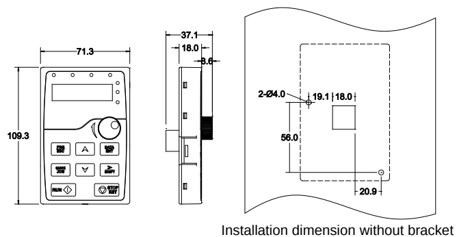
Installation dimension without bracket
